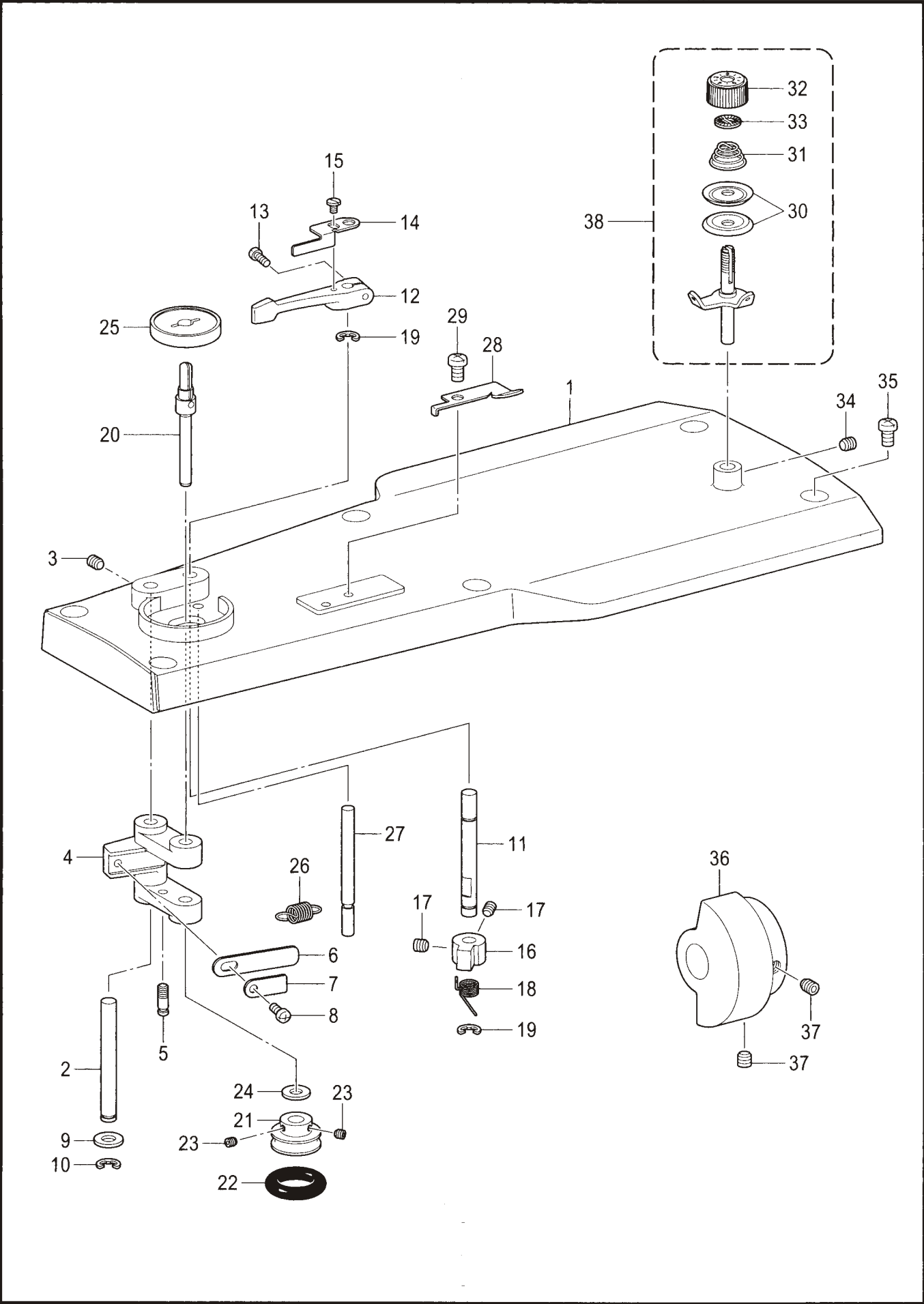
J. 卷线装置 / Bobbin winder mechanism
