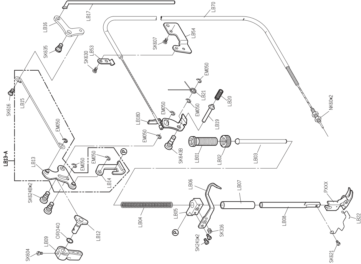
PARTS LIST FOR LB GROUP
